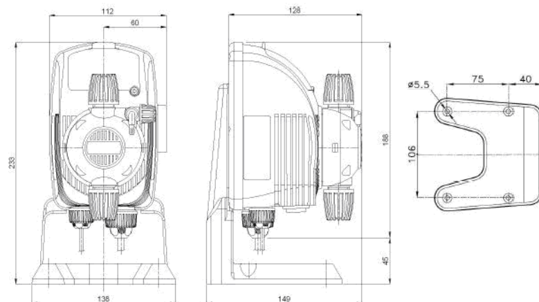
Figure 2: When used with horizontal mount bracket
