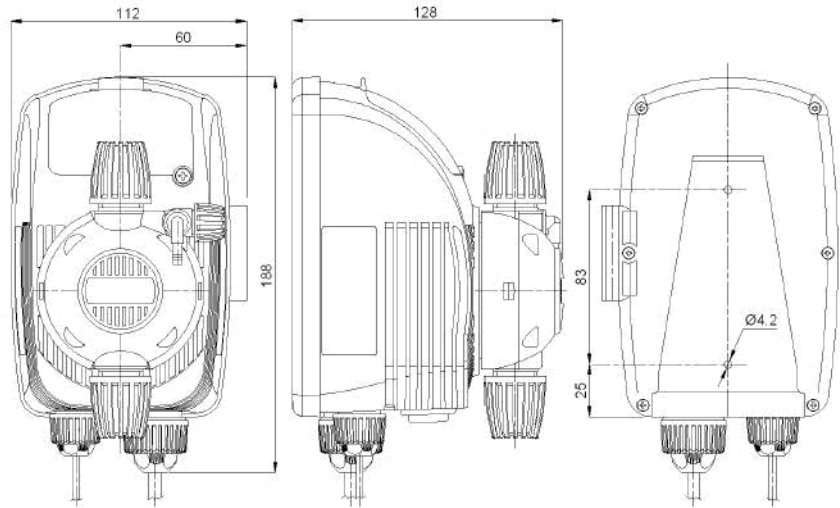
Figure 1: When used with vertical mount bracket
